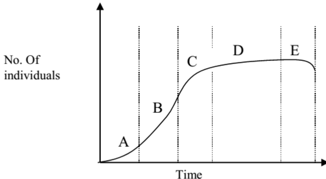
The population growth curve
